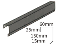
Barge Board Cover 山墙板
