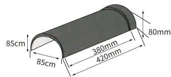
Circular Ridge Cap 圆弧脊瓦
